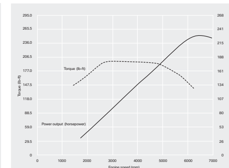
Portrait of an engineering masterpiece: the 3.0-liter engine pours on the power and quickly develops maximum torque, which continues without fading over a large rpm range – so you enjoy smooth, powerful acceleration at virtually any legal speed.
