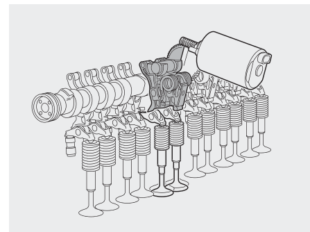
BMW's Valvetronic system reduces "pumping losses" in the engine, especially under part-load conditions, thereby reducing fuel consumption.
